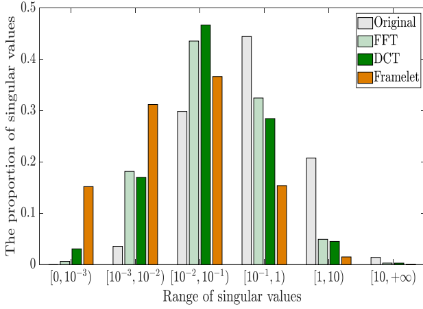
Fig. 2. The distribution of singular values. Here, the singular values are obtained by conducting SVD on each frontal slice of the original tensor data or the transformed tensors.
