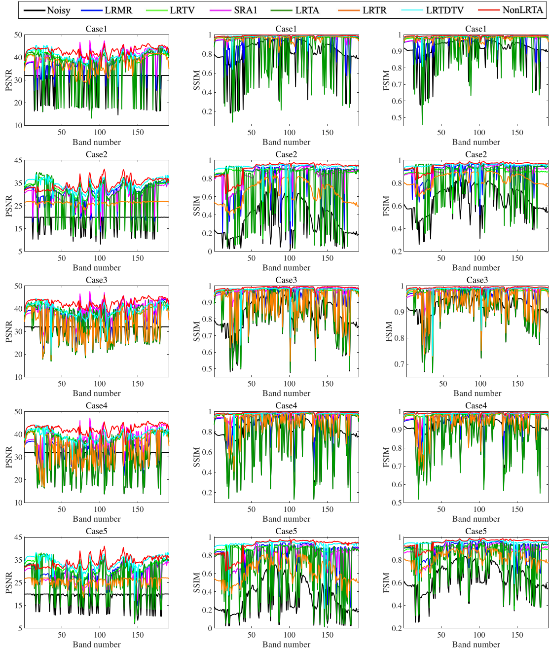
Fig. 2. PSNR, SSIM and FSIM values of each band in simulated experiment. The first to the fifth rows correspond to simulated experiments cases 1 to 5, respectively.
