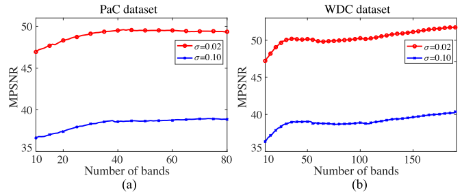
Fig. 21. Influence of the number of spectral bands on the denoising effect. (a) PaC data set. (b) WDC data set.
