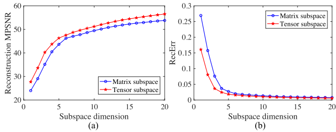
Fig. 20. Presentation capability comparison of the matrix and tensor subspace. (a) Reconstruction MPSNR with respect to the subspace dimension. (b) RecErr with respect to the subspace dimension.
