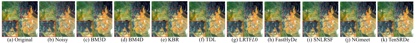
Fig. 13. (a) Original pseudocolor image (R: 80, G: 140, B: 180) of the Cuprite data set. (b) Noisy image with the Gaussian noise level \sigma = 0.10 . Denoised results of (c) BM3D, (d) BM4D, (e) KBR, (f) TDL, (g) LRTFL0, (h) FastHyDe, (i) SNLRSF, (j) NGmeet, and (k) TenSRDe. To facilitate the observation of details, the demarcated area in each image is enlarged.
