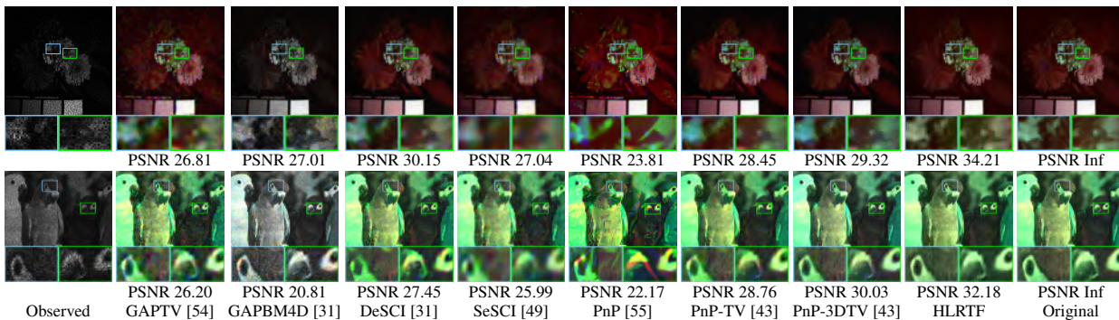
Figure 7. The results of snapshot spectral imaging by different methods on MSI Flowers and MSI Bird (SR = 0.5).
