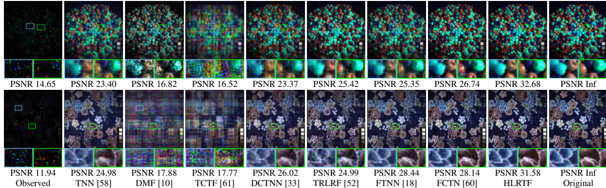
Figure 5. The results of multi-dimensional image completion by different methods on MSI Beans and MSI Cloth (SR = 0.1).
