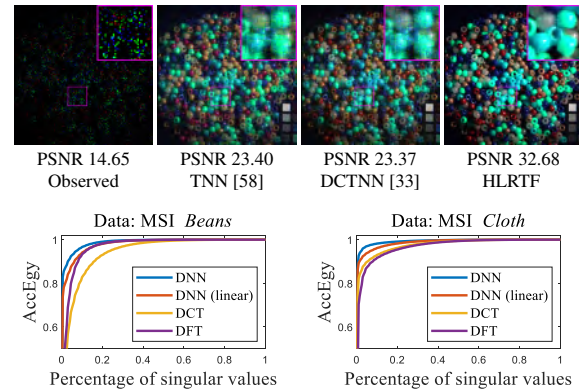
Figure 1. Top: The results of multi-dimensional image completion by TNN (based on the DFT) [58], DCTNN (based on the DCT) [33], and HLRTF (based on the DNN transform) on MSI Beans with sampling rate 0.1. Bottom: The AccEgy (AccEgy = \sum_{i=1}^k \sigma_i^2 / \sum_j \sigma_j^2 with \sigma_i denotes the i -th singular value [46]) versus the percentage of singular values of the transformed frontal slices by different transforms (i.e., the DNN transform, the DNN transform with only one layer, the DCT, and the DFT). The DNN transform obtains lower-rank transformed frontal slices and thus the corresponding HLRTF achieves better recovery performance.
