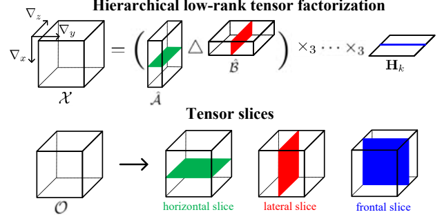
Figure 3. Figurative expressions of Lemma 2. (i) If the i -th horizontal slice of \mathcal{O} is missed, then the gradient on the i -th horizontal slice of \hat{\mathcal{A}} equals to zero. (ii) If the i -th lateral slice of \mathcal{O} is missed, then the gradient on the i -th lateral slice of \hat{\mathcal{B}} equals to zero. (iii) If the i -th frontal slice of \mathcal{O} is missed, then the gradient on the i -th row of \mathbf{H}_k equals to zero.
