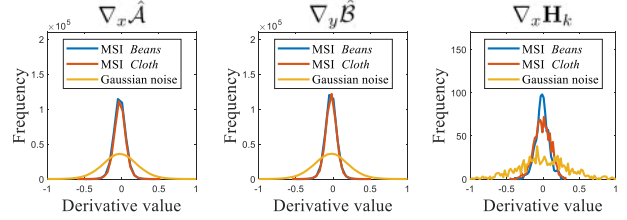
Figure 4. The statistical distributions of derivative values of factors for different data \mathcal{O} : the ground-truth MSI Beans, the ground-truth MSI Cloth, and the Gaussian noise. Given the data \mathcal{O} , the factors are obtained by optimizing (3) using the Adam.
