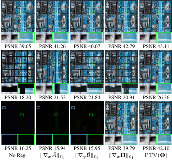
Figure 2. The results of multi-dimensional image completion on HSI WDC mall with random missing (first row), horizontal/lateral slice missing (second row), and frontal slice missing (third row) by HLRTF with different regularizations.
