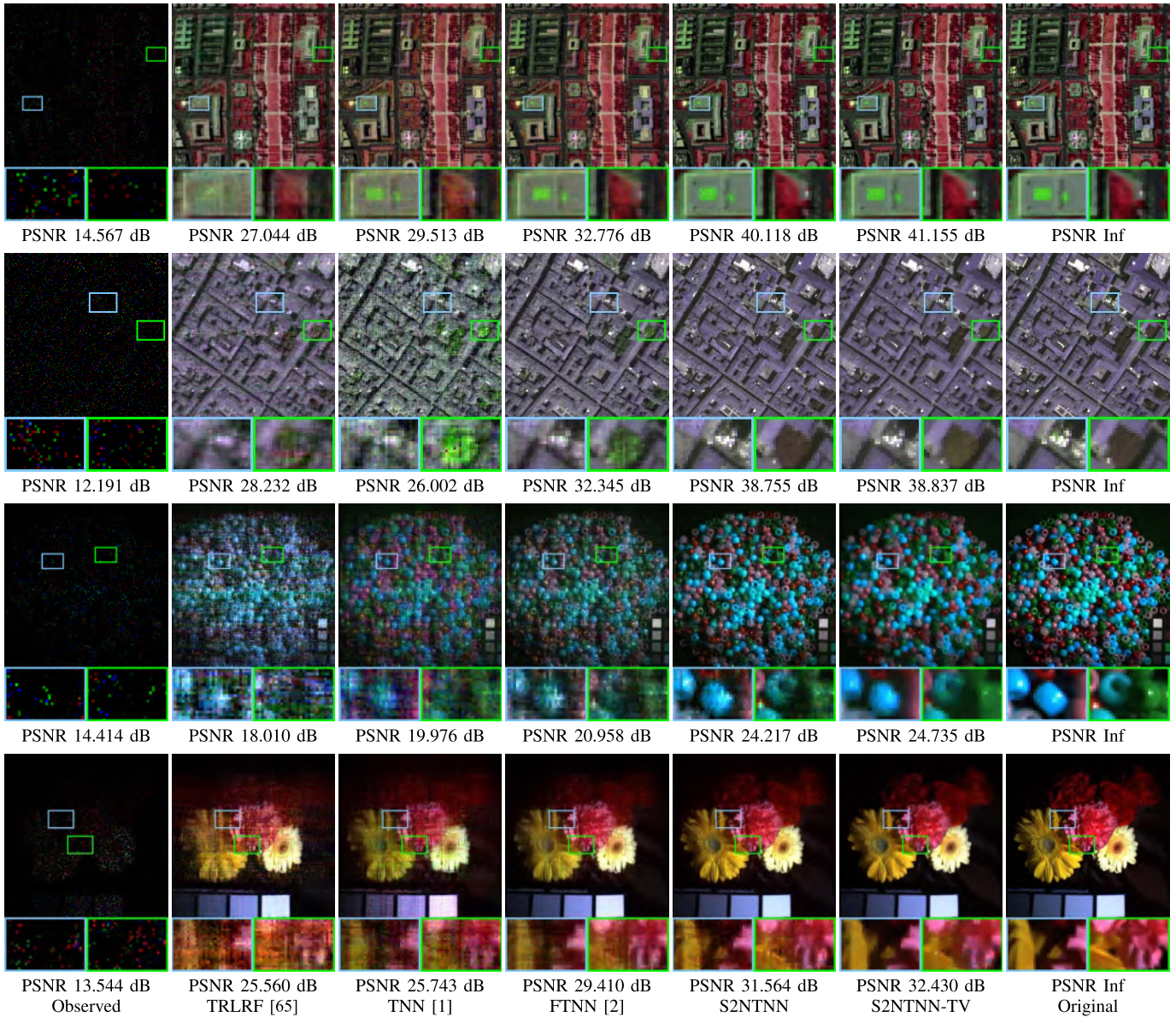
Fig. 5. The recovered results by different methods for tensor completion on HSI WDC mall (composed of the 50-th, 100-th, and the 150-th bands) with SR = 0.05 , HSI Pavia (composed of the 1-st, 10-th, and the 20-th bands) with SR = 0.05 , MSI Beads (composed of the 10-th, 20-th, and the 30-th bands) with SR = 0.05 , and MSI Flowers (composed of the 10-th, 20-th, and the 30-th bands) with SR = 0.05 .
