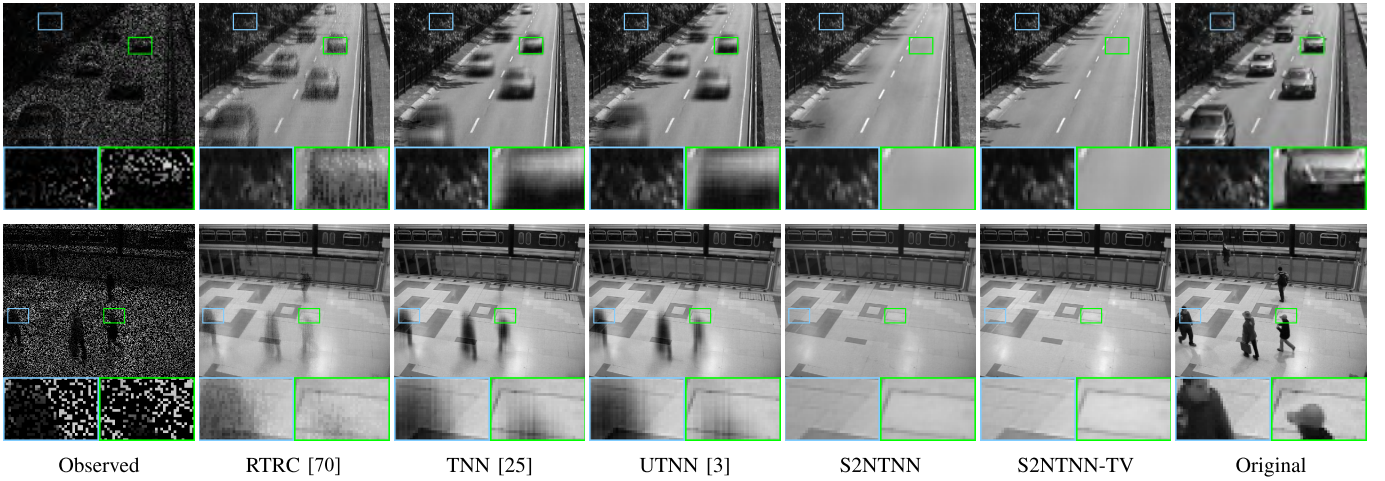
Fig. 8. The separated background by different methods for RTC on videos highway ( 240 \times 320 \times 200 ) and PET ( 288 \times 360 \times 300 ) with SR = 0.25 .
