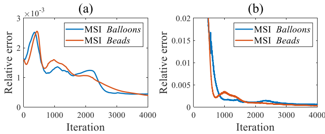
Fig. 13. The relative error with respect to iterations for tensor completion with SR = 0.25 . (a) The relative error of f and g parameters, i.e., \sum_{i=1}^{p+q} \|\mathbf{W}_i^{t+1} - \mathbf{W}_i^t\|_F^2 / \|\mathbf{W}_i^t\|_F^2 . (b) The relative error of \mathcal{V}_d , i.e., \sum_{d=1,2} \|\mathcal{V}_d^{t+1} - \mathcal{V}_d^t\|_F^2 / \|\mathcal{V}_d^t\|_F^2 .
