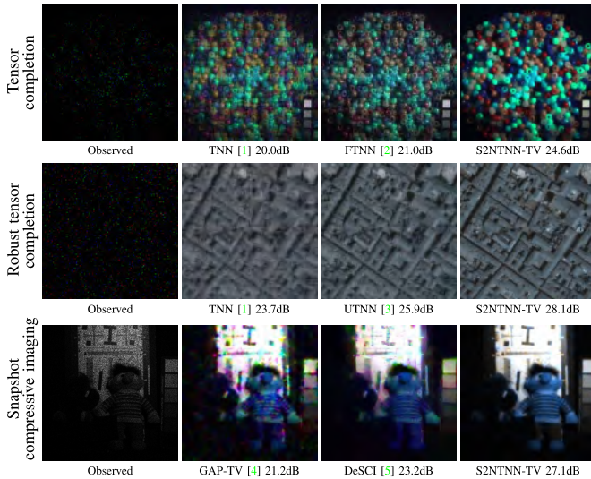
Fig. 1. The recovered results and PSNR values by different methods. Three rows respectively list the recovered results for tensor completion on MSI Beads with SR = 0.05 , the recovered results for robust tensor completion on HSI Pavia with SR = 0.05 , and the recovered results for snapshot compressive imaging on MSI Toys with SR = 0.25 . The proposed S2NTNN-TV obtains the best PSNR values and qualitative results compared with state-of-the-art methods.
