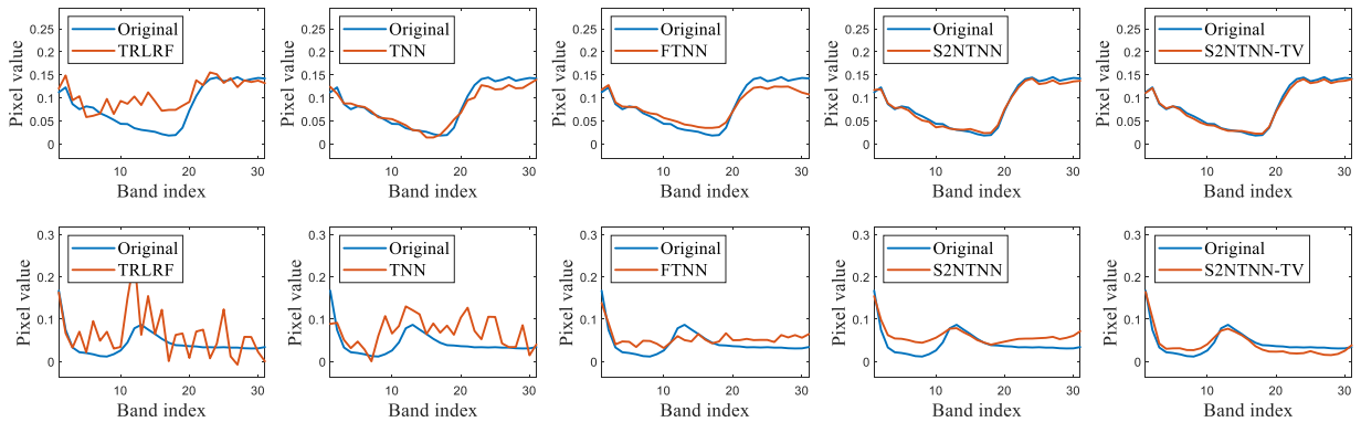
Fig. 4. The spectral curves of the tensor completion results by different methods on MSIs Balloons and Beads with SR = 0.05.
