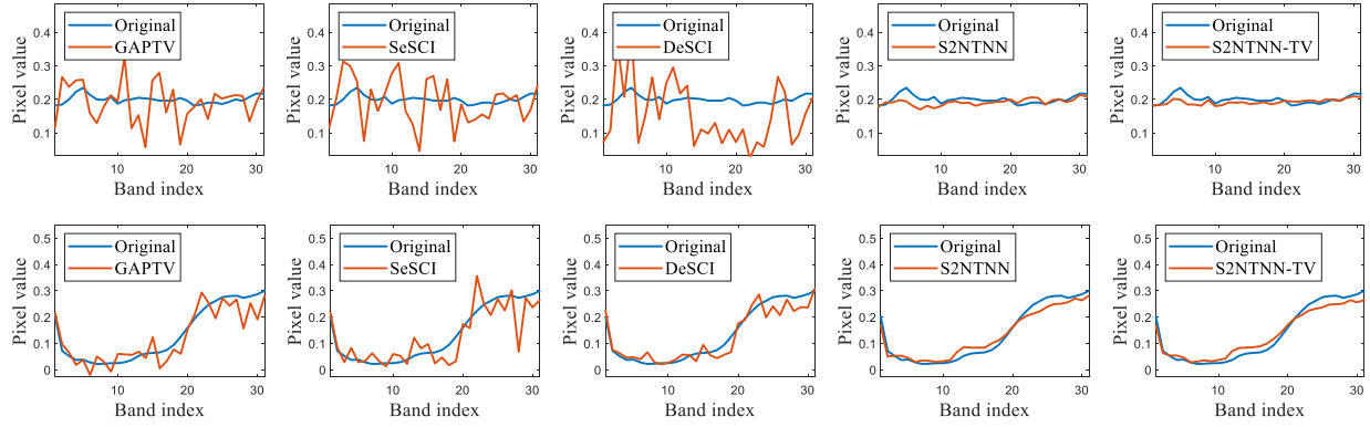
Fig. 10. The spectral curves of recovered results by different methods for SCI on MSIs Toys and Flowers with SR = 0.25 .
