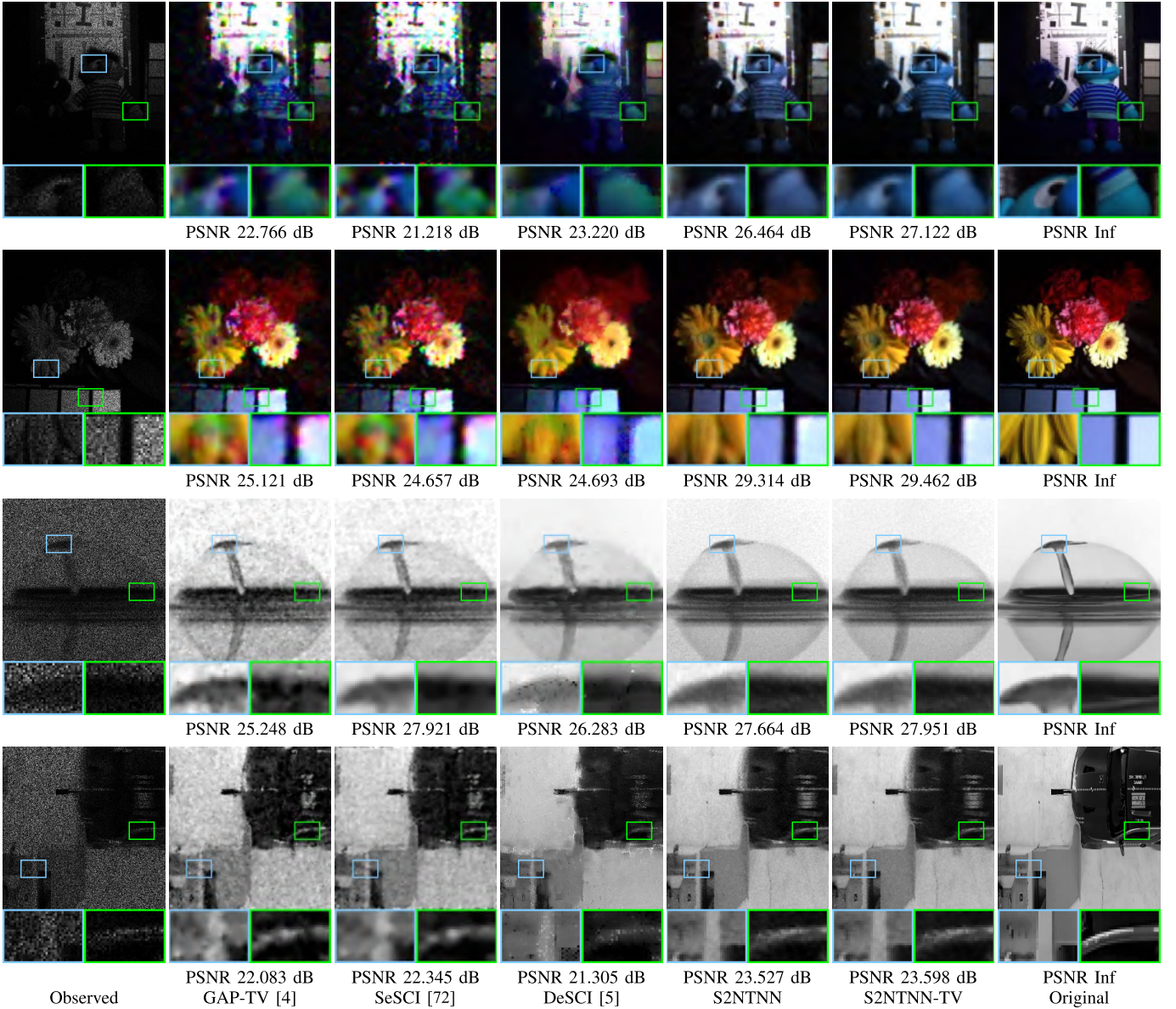
Fig. 9. The recovered results by different methods for SCI on MSI Toys (composed of the 10-th, 20-th, and the 30-th bands) with SR = 0.25 , MSI Flowers (composed of the 10-th, 20-th, and the 30-th bands) with SR = 0.25 , video Drop with SR = 0.25 , and video Crash with SR = 0.25 .
