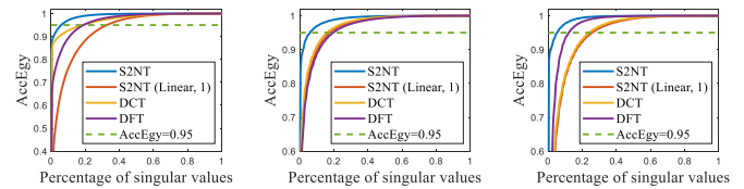
Fig. 2. The accumulation energy ratio (AccEgy) [31] with respect to the percentage of singular values of the transformed frontal slices of HSI Pavia , HSI WDC mall , and MSI Beads . The AccEgy is defined as \sum_{i=1}^k \sigma_i^2 / \sum_j \sigma_j^2 , where \sigma_i is the i -th singular value. We can observe that S2NT obtains a better low-rank representation whose energy is concentrated in the larger singular values. Thus, the corresponding S2NTNN could achieve more promising results.
