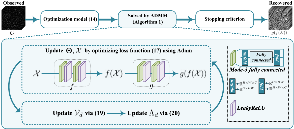
Fig. 3. The pipeline of the proposed S2NTNN-TV for multi-dimensional image recovery. Compared with traditional linear transform-based TNN family methods, our method employs nonlinear transforms f and g with high representation abilities to help obtain a better low-rank representation, leading to a promising improvement of the recovery performance.
