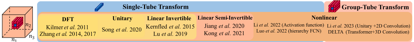
Fig. 1. Representative works on transforms within the t-SVD framework.
